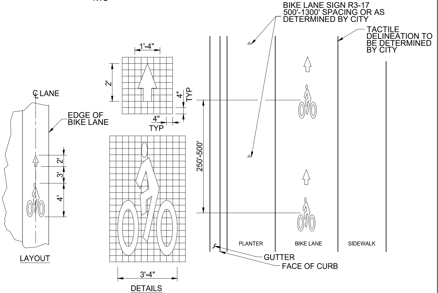
TYPICAL PROTECTED BICYCLE LANE NTS
