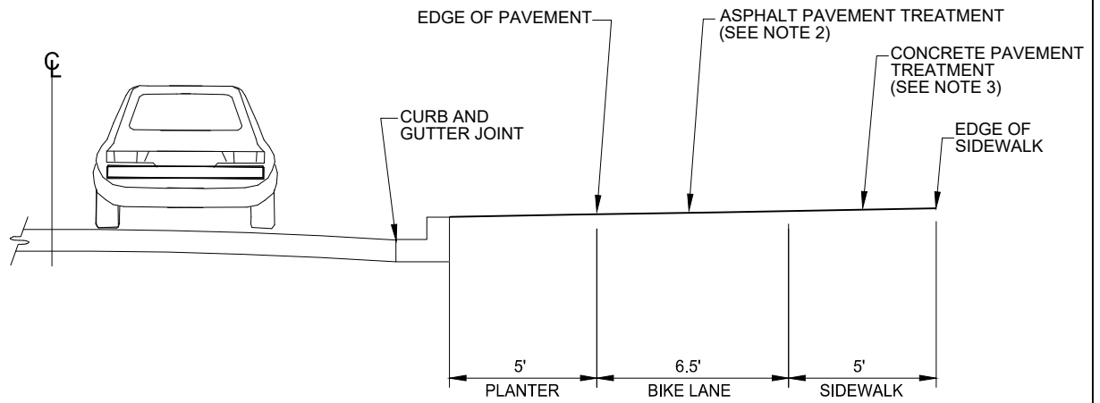
PROTECTED BICYCLE LANE NTS
